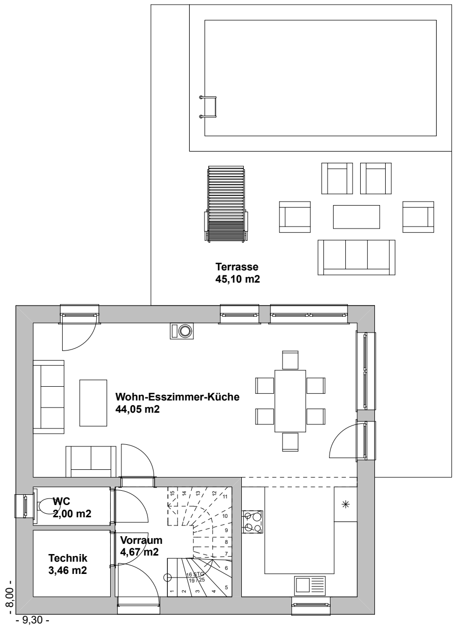
Erdgeschoss M 1:100 - WNF = 54,18 m 2
