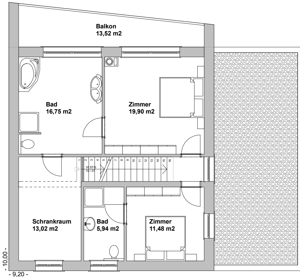
Obergeschoss M 1:100 - WNF = 69,13 m
